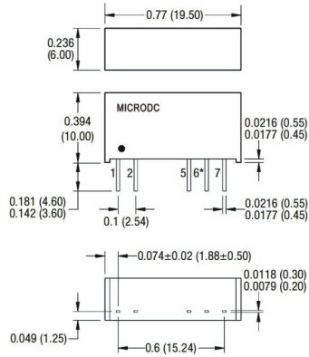
SIP package
